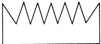
FIG. 2 — A polygon with many ears.
